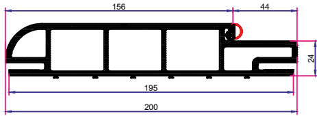
OVAL 200 mm KAPI KASA
