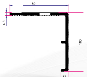
80x100 mm PERVAZ
